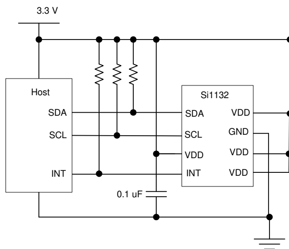
Figure 1. Si1132 Application
